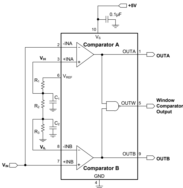
Figure 2. Window Comparator
