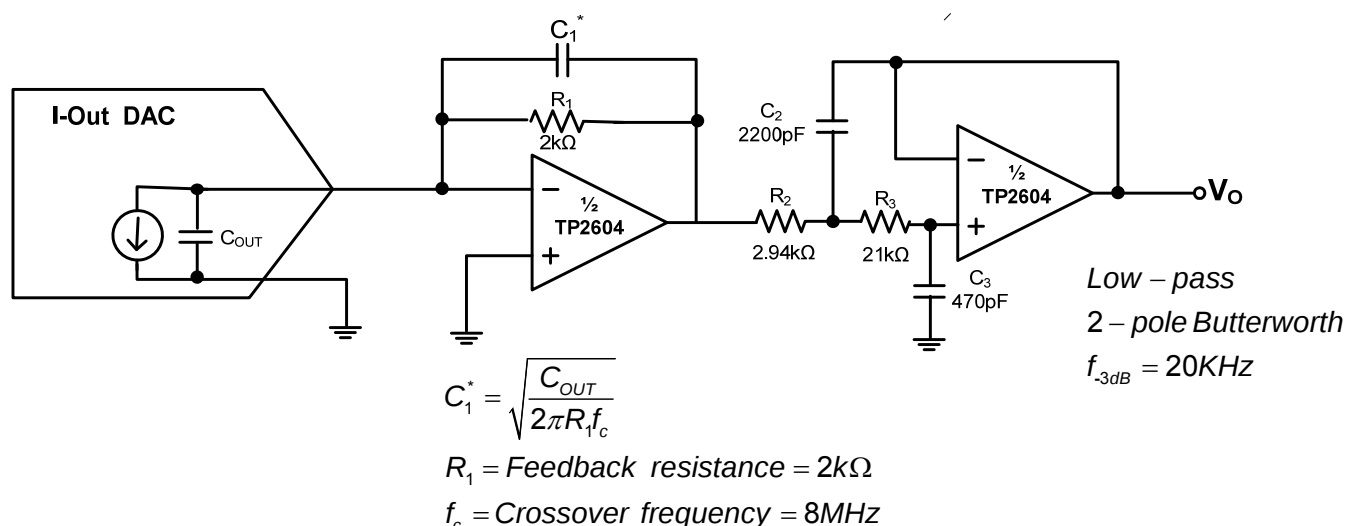
Figure 5 DAC I/V Amplifier and Low-Pass Filter
