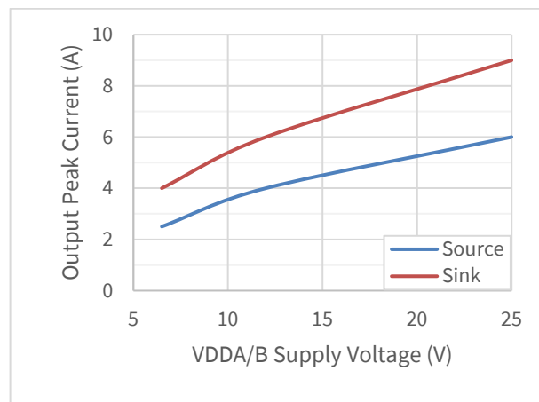
Figure 5.8 Output Peak Current vs VDDA/B Supply Voltage
