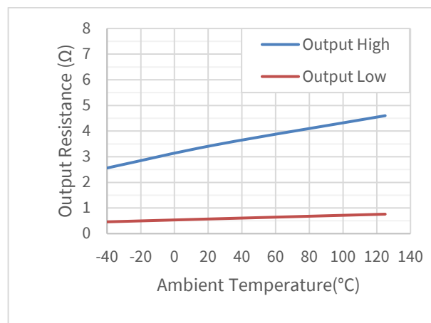
Figure 5.6 Output Resistance vs Temperature
