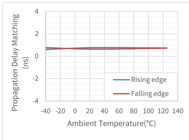
Figure 5.19 Propagation Delay Matching vs Temperature
