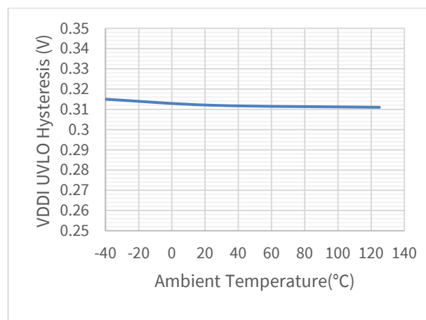
Figure 5.12 6V VDDA/B UVLO Hysteresis vs Temperature
