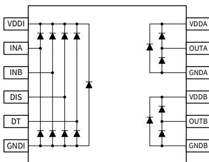
Figure 7.3 ESD Structure
