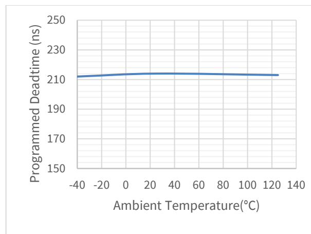
Figure 5.22 Deadtime (RDT=20kΩ) vs Temperature
