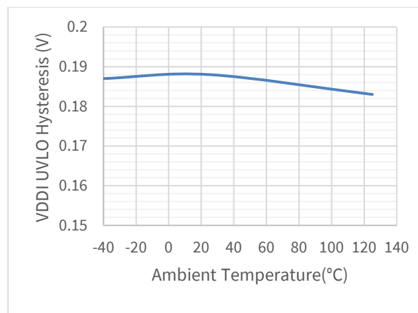
Figure 5.10 VDDI UVLO Hysteresis vs Temperature
