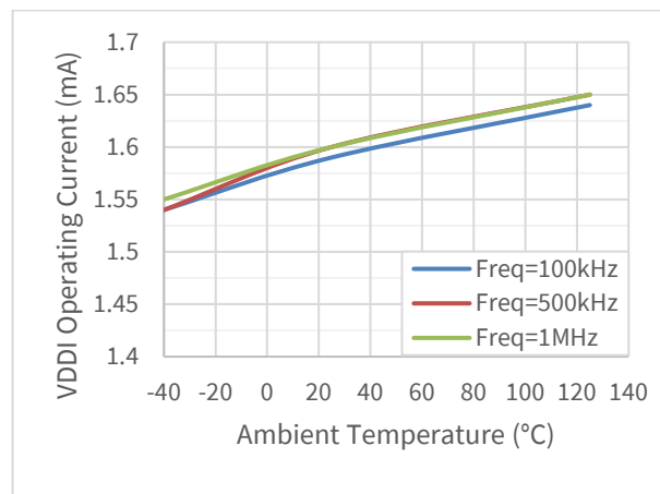
Figure 5.2 VDDI Operating Current vs Temperature
