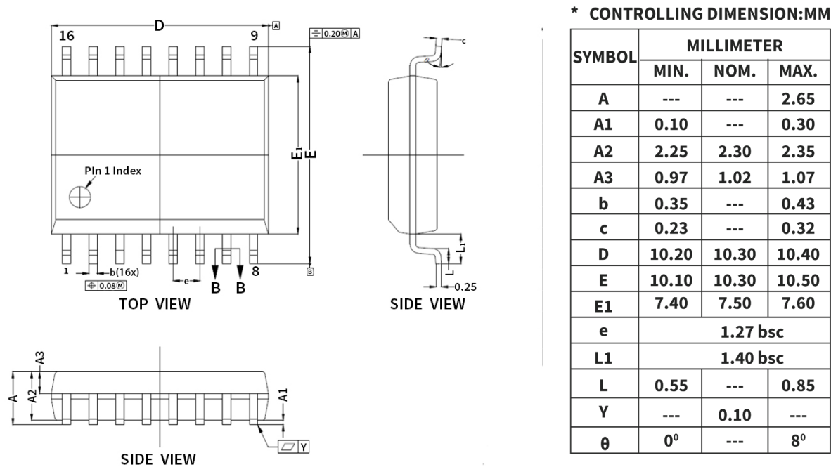
Figure 9.3 SOW16 Package Shape and Dimension
