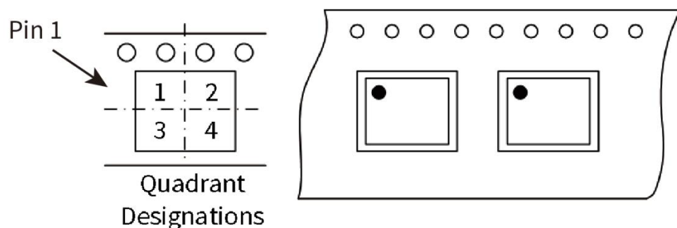
Figure 11.5 Quadrant Designation for Pin1 Orientation in Tape
