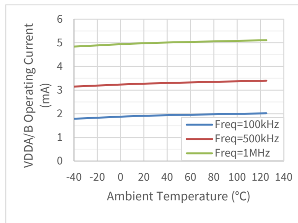
Figure 5.4 VDDA/B Operating Current vs Temperature
