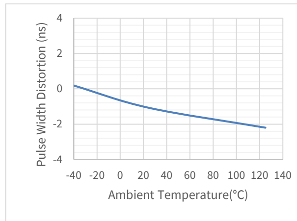
Figure 5.20 Pulse Width Distortion vs Temperature
