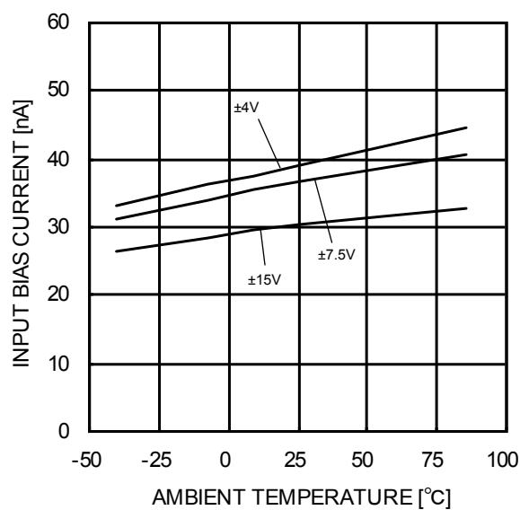
Figure 13. Input Bias Current - Ambient Temperature ( V_{ICM}=0V , V_{OUT}=0V )
