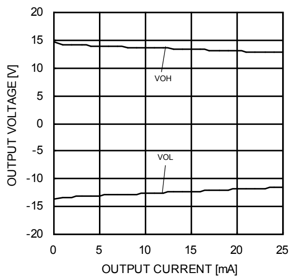
Figure 31. Maximum Output Voltage - Output Current ( V_{CC}/V_{EE}=+15V/-15V , T_A=25^\circ\text{C} )
