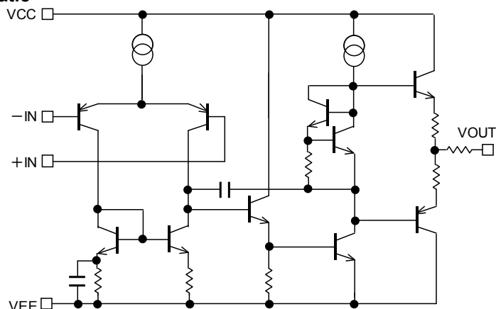
Figure 1. Simplified Schematic
