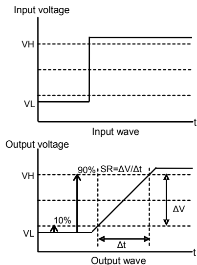
Figure 92. Slew Rate Input/Output Waveform
