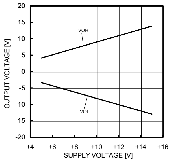
Figure 29. Maximum Output Voltage - Supply Voltage ( R_L=2k\Omega , T_A=25^\circ\text{C} )
