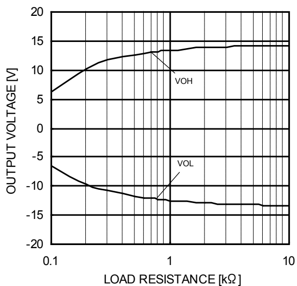
Figure 28. Maximum Output Voltage - Load Resistance ( V_{CC}/V_{EE}=+15V/-15V , T_A=25^\circ\text{C} )
