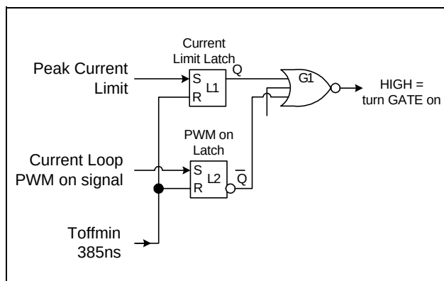
Figure 13 PWM Logic
