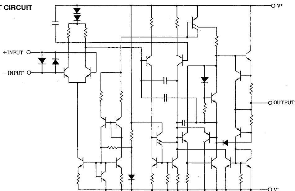
NJM5532D NJM5532M
