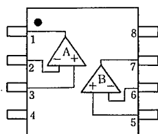
NJM5532D NJM5532M
