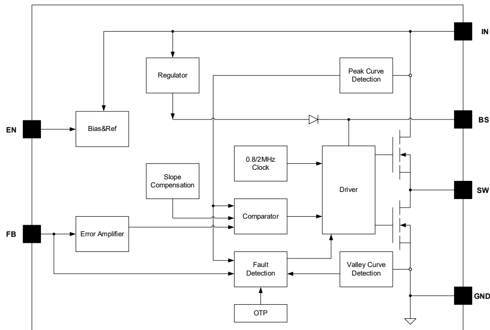
Block Diagram
