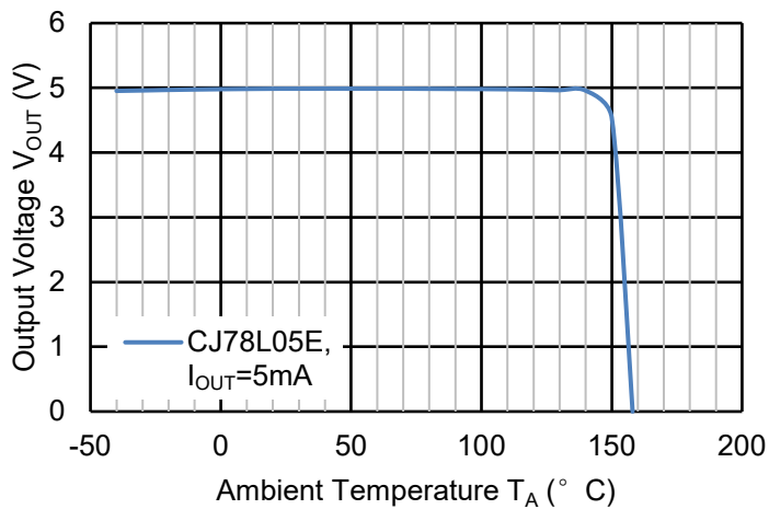
Thermal Shutdown
