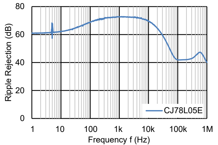
Ripple Rejection
