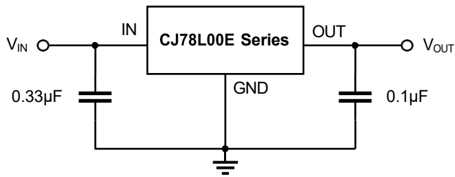
Figure 9-1. Conventional Circuit
