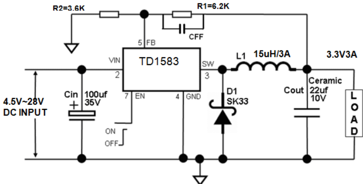
Fig11. TD1583 Typical Application Circuit (with ceramic output capacitor) @ 3.3V/3A
