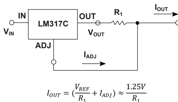
Figure 9-4. Current Regulator
