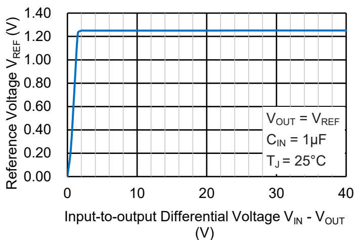
Line Regulation
