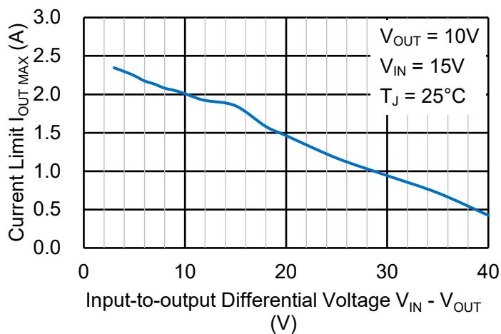
Current Limit
