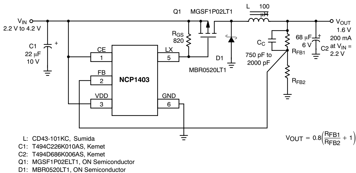
Figure 34. Step-down DC-DC Converter with 1.6 V Output Voltage for DSP Circuit
