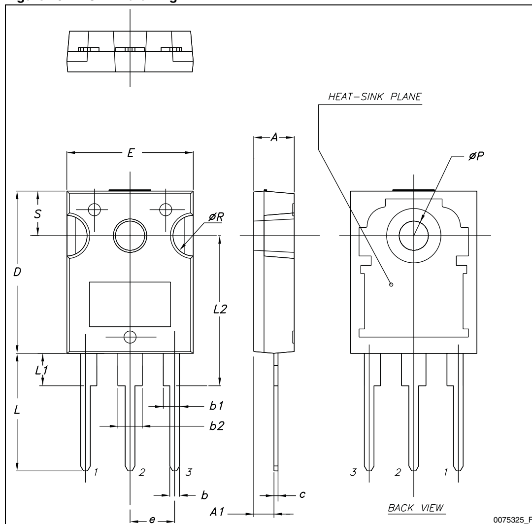
Figure 26. TO-247 drawing
