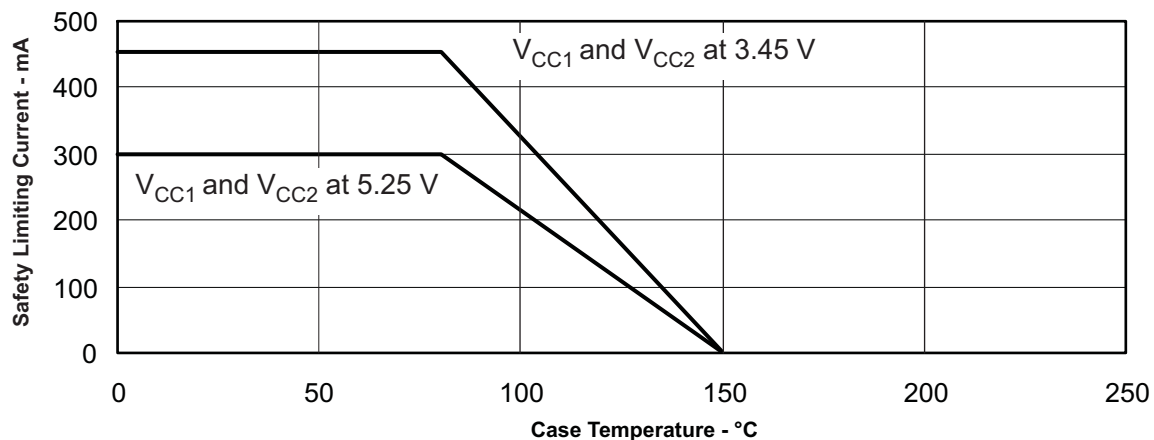
Figure 8. DW-16 R_{OJC} Thermal Derating Curve for VDE
