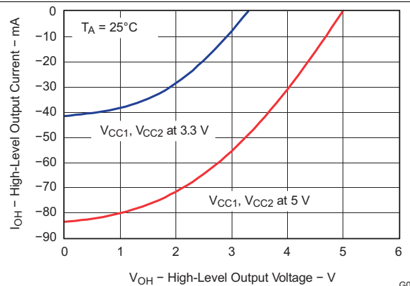
Figure 2. High-Level Output Current vs High-Level Output Voltage
