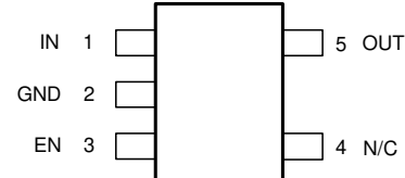
Figure 4-3. DBV Package, 5-Pin SOT-23 (Top View)
