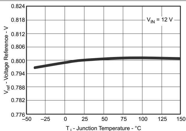
图 6-4. Voltage Reference vs Junction Temperature
