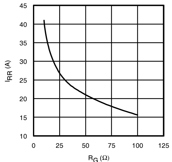
Fig. 18 - Typ. Diode I_{\text{RR}} vs. R_G T_J = 175^\circ\text{C}
