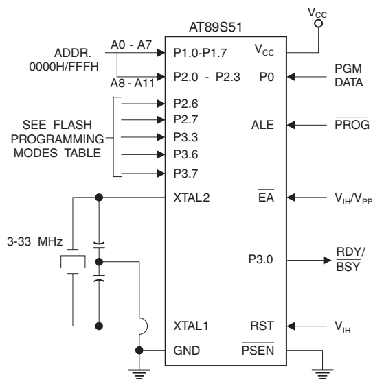
Figure 17-1. Programming the Flash Memory (Parallel Mode)
