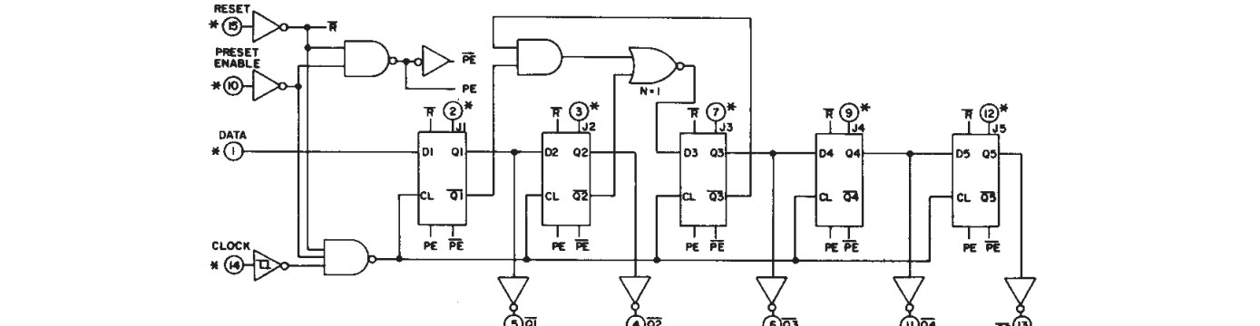
Fig. 1 – Logic diagram
