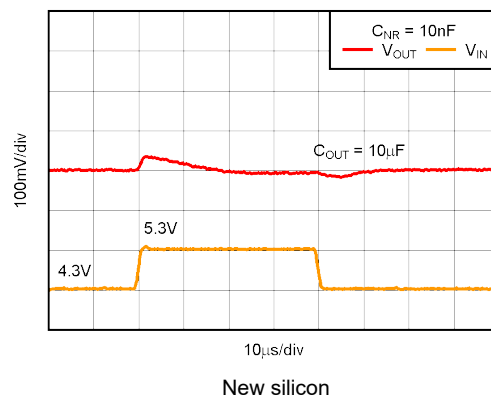
图 5-38. TPS73733 Line Transient Response
