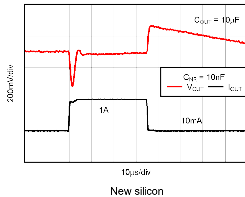
图 5-36. TPS73733 Load Transient Response
