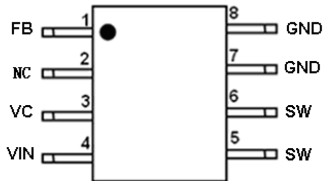
Figure2. Pin Configuration of XL2001 (Top View)
