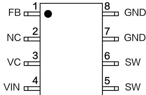
Figure2. Pin Configuration of XL2011 (Top View)
