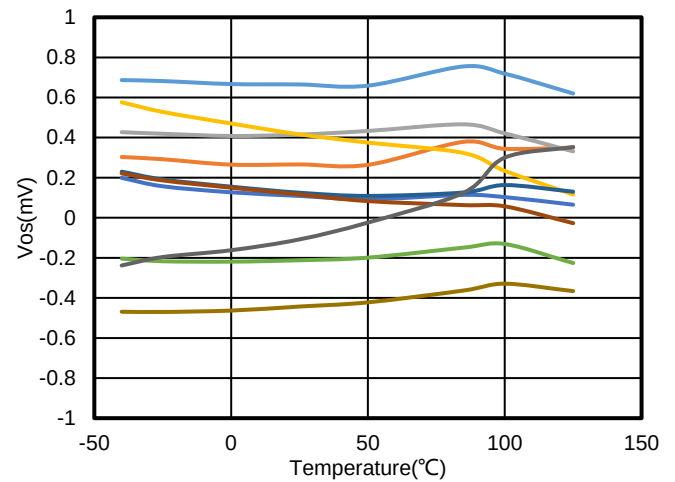
Figure 2. Vos vs. Temperature, 10ch Data
