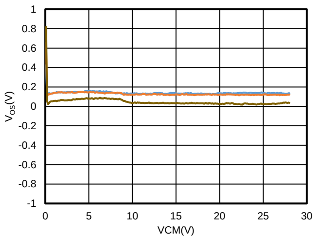
Figure 3. Offset Voltage vs. Common Mode Voltage, 3ch Data
