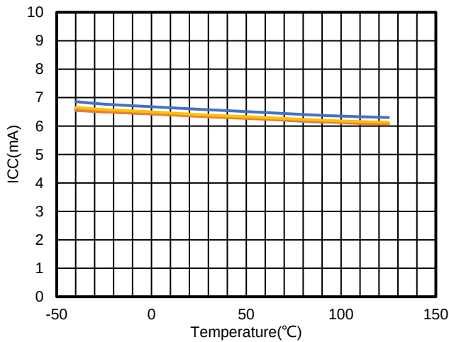
Figure 1. Quiescent Current vs. Temperature, TP2582, 3 Samples
