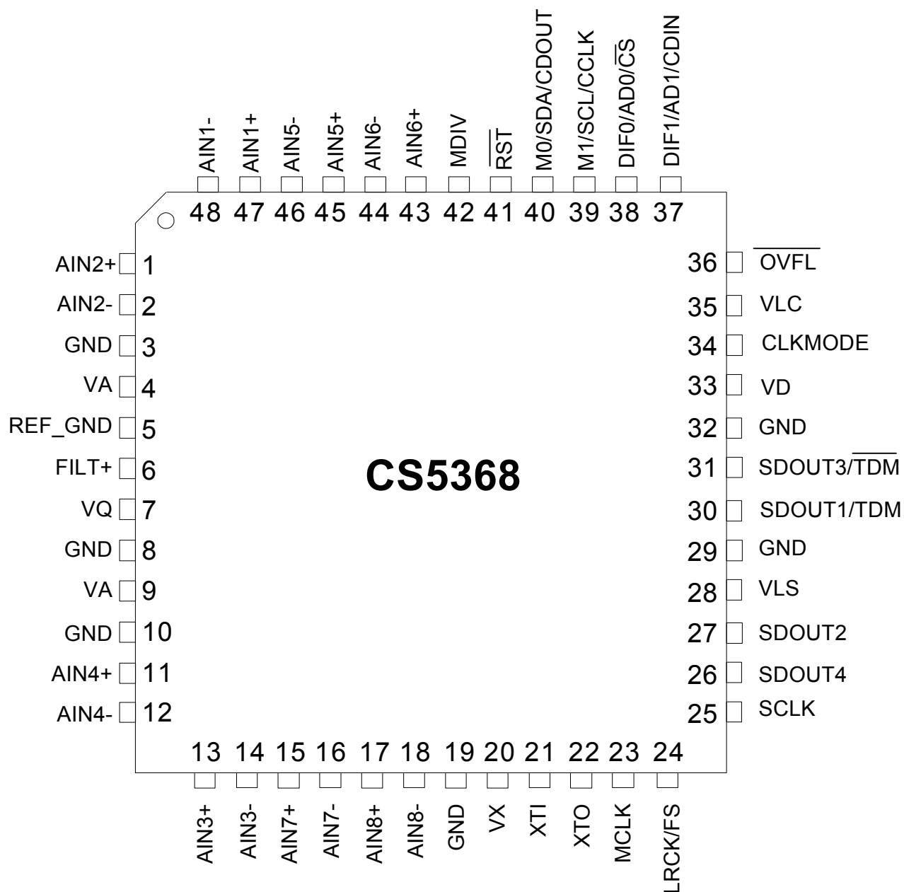
Figure 1. CS5368 Pinout
