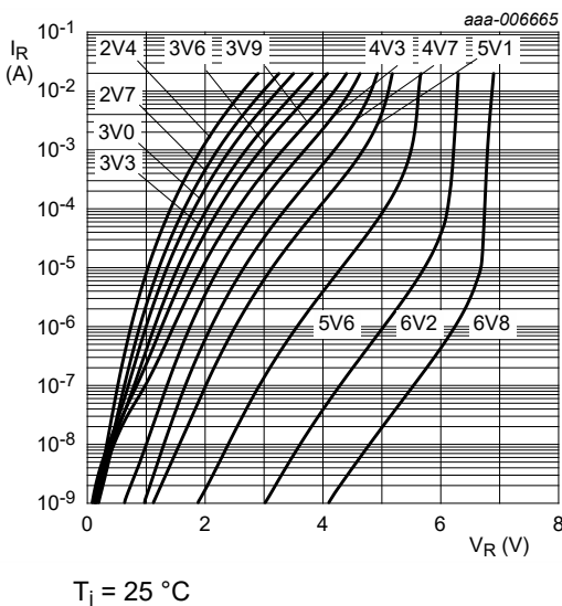
Fig. 8. Reverse current as a function of reverse voltage; typical values (BZX384-A/B/C2V4 to BZX384-A/B/C6V8)
