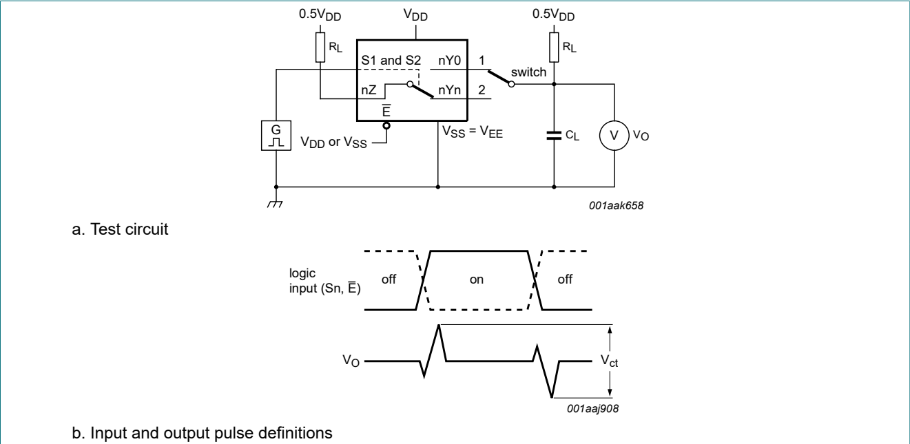
Fig. 20. Test circuit for measuring crosstalk voltage between digital inputs and switch
