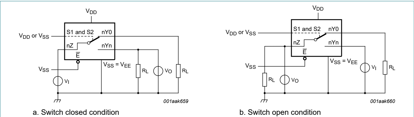
Fig. 21. Test circuit for measuring crosstalk between switches
