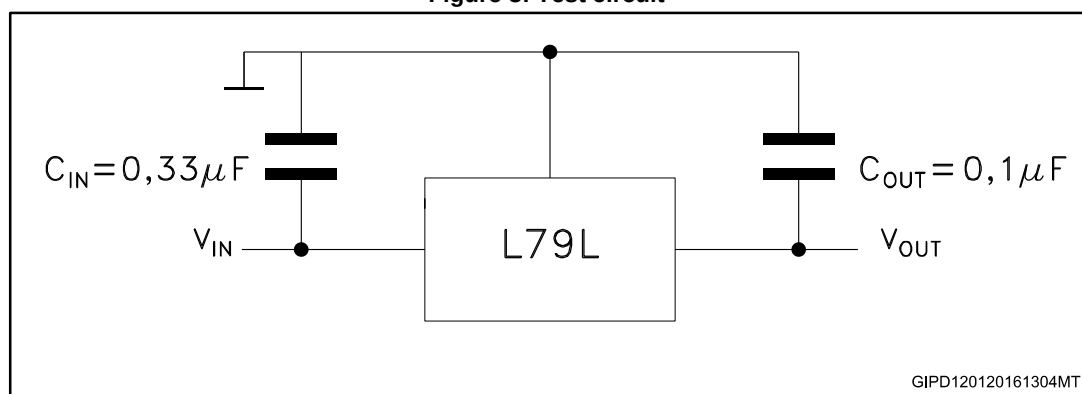
Figure 3: Test circuit
