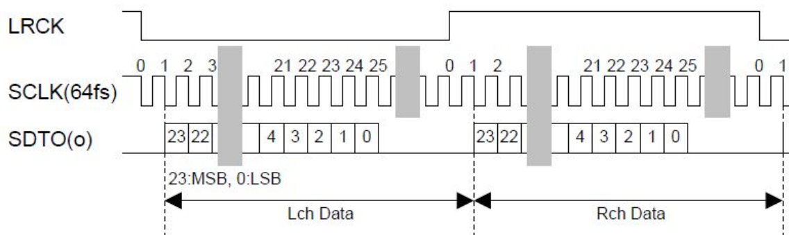
Figure 2. Mode 1 Timing
