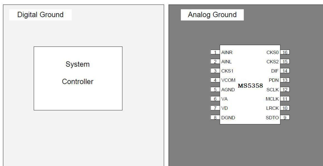
Figure 6. Ground Layout
