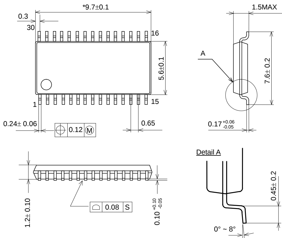
30pin VSOP (Unit: mm)
