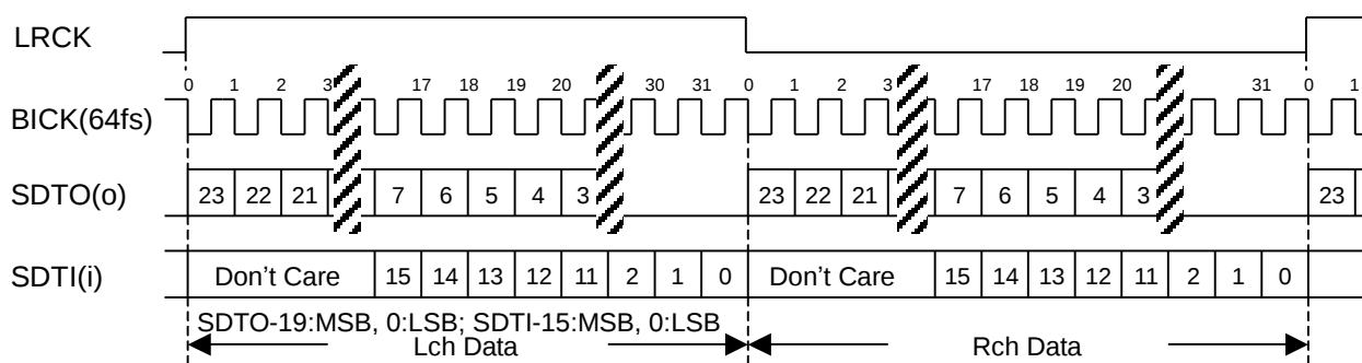
Figure 7. Mode 0 Timing
