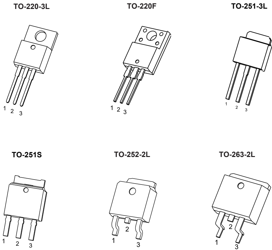
Figure 6-1. Pin Configuration
