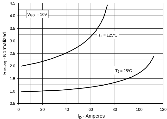
Fig. 5. R_{DS(on)} Normalized to I_D = 23A Value vs. Drain Current
