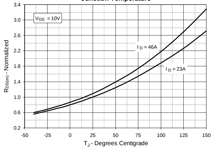
Fig. 4. R_{DS(on)} Normalized to I_D = 23A Value vs. Junction Temperature
