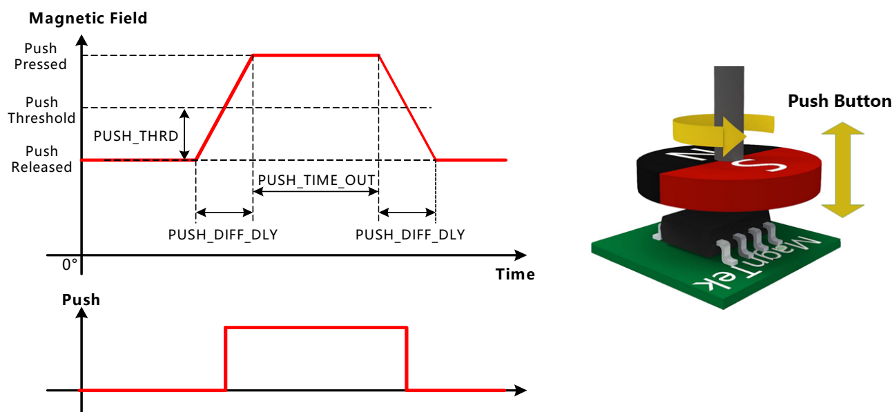
Figure 26: Pushbutton Function
