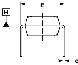
END VIEW WITH LEADS CONSTRAINED NOTE 5
