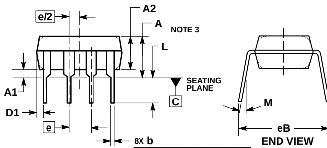
END VIEW NOTE 6
