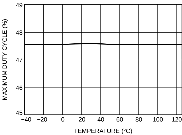
Figure 18. Maximum Duty-cycle, A Version vs. Junction Temperature
