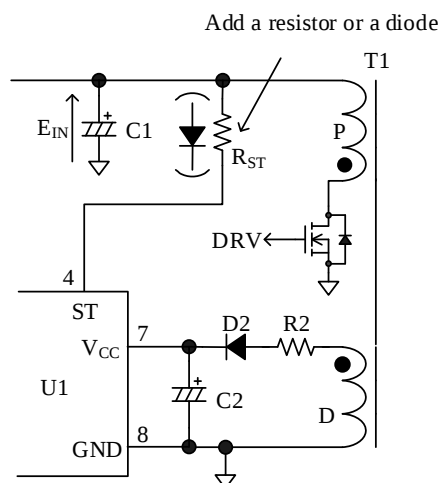
Figure 9-3. ST Pin Countermeasure against Negative Applied Voltage
