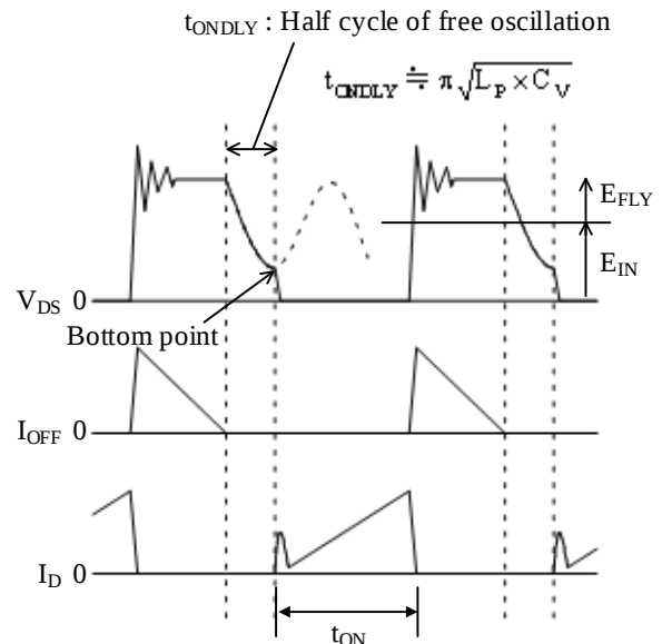
Figure 8-12. Ideal bottom-on operation waveform (Power MOSFET turn-on at a bottom point of a V_{DS} waveform)
