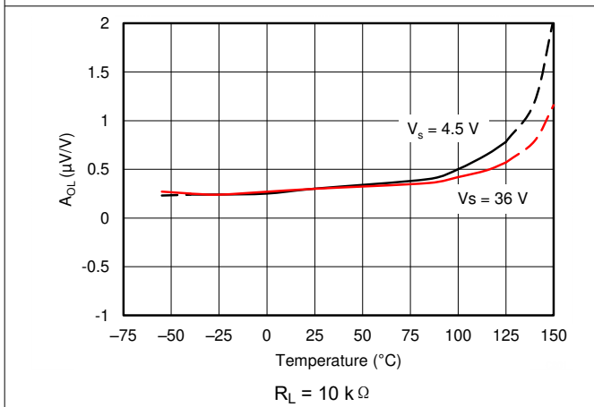
图 7-23. Open-Loop Gain vs Temperature
