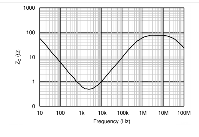
图 7-24. Open-Loop Output Impedance vs Frequency
