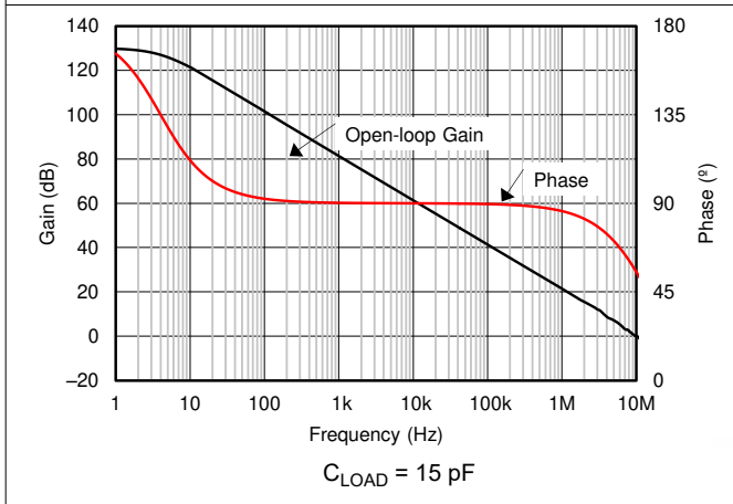
图 7-21. Open-Loop Gain and Phase vs Frequency
