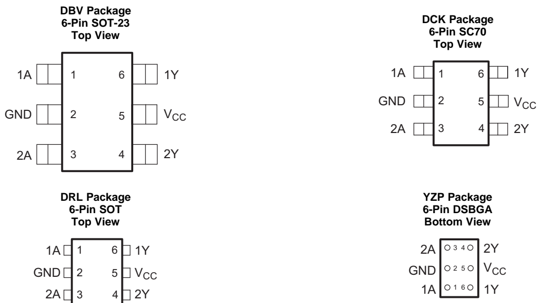
Pin Functions (1)
