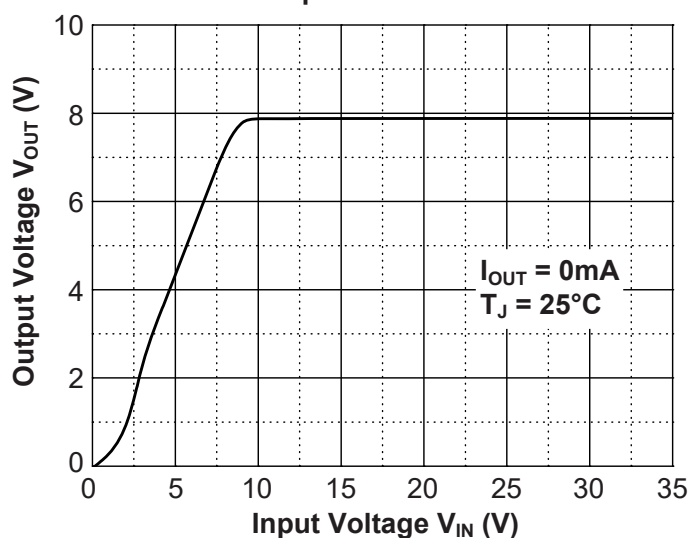
Output Characteristics
