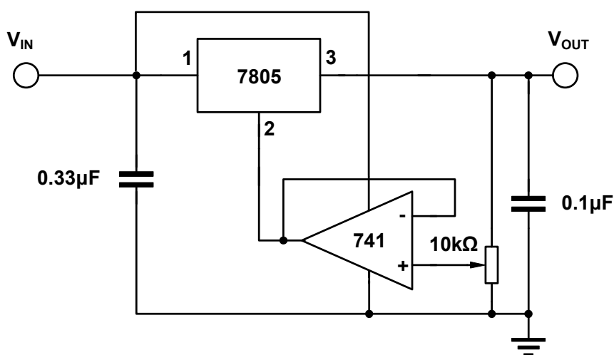
Figure 9-13. Adjustable Output
