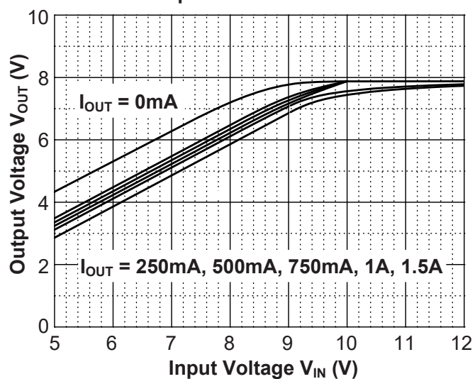
Dropout Characteristics
