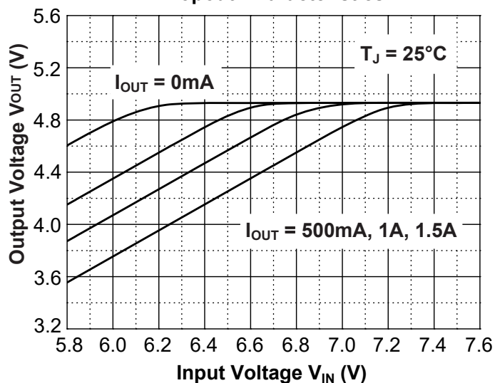
Dropout Characteristics
