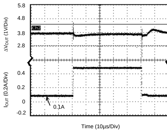
Load Transient Response (Conditions: V_{IN} = 4.8 V, V_{OUT} = 3.33 V, I_{OUT} = 0.1 to 0.5 A, C_{IN} = C_{OUT} = 10 μF)
