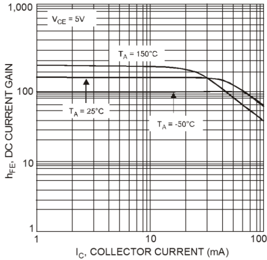
Figure 2. DC Current Gain vs. Collector Current
