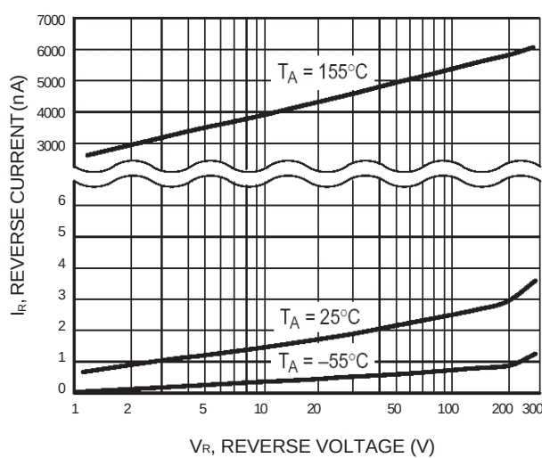
Figure 2. Reverse Leakage
