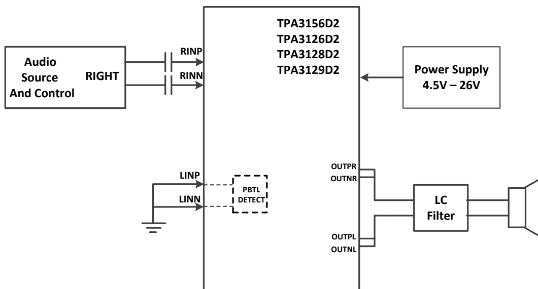
Figure 32. PBTL Mode
