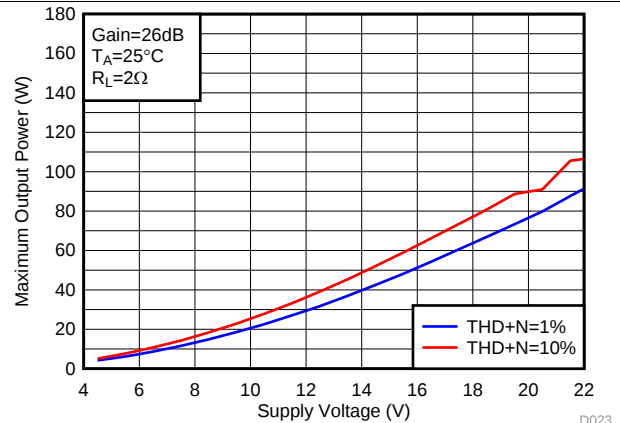
Figure 20. Maximum Output Power (PBTL) vs Supply Voltage
