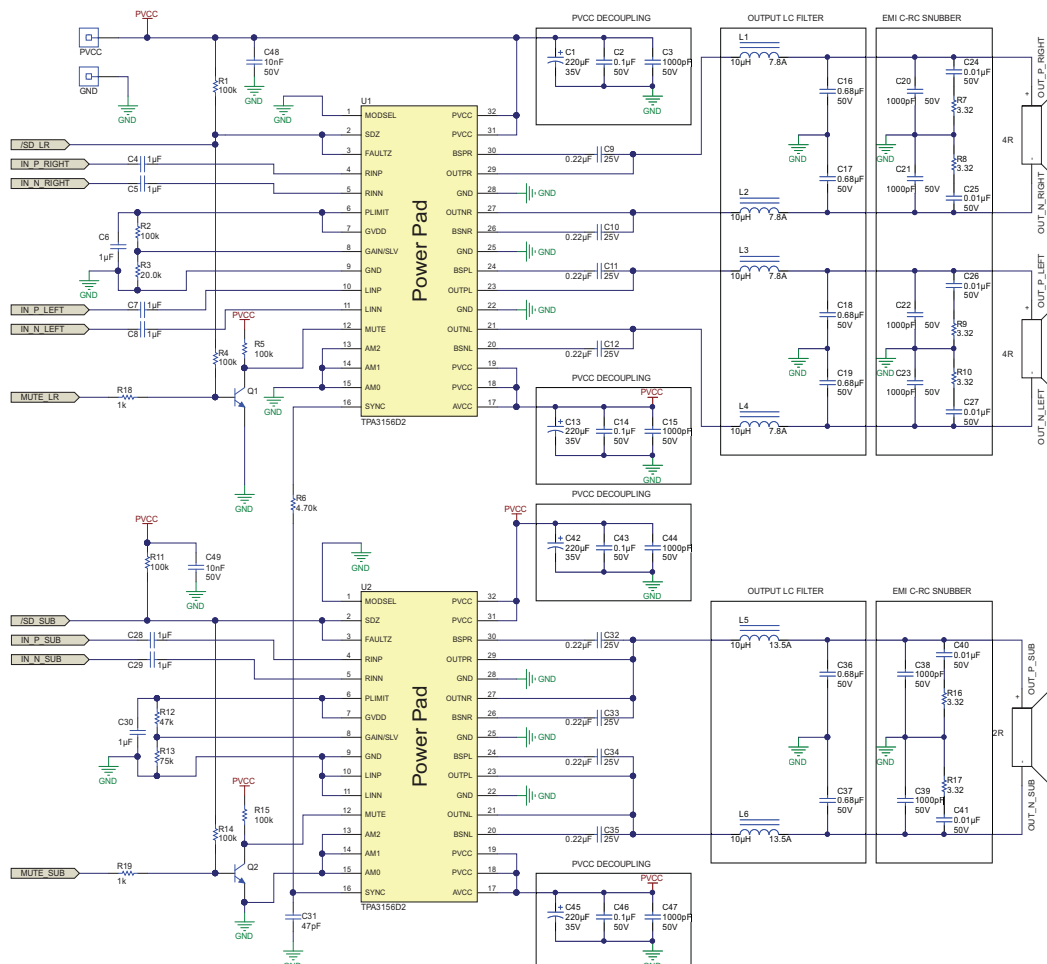
Figure 34. TPA3156D2 Schematic
