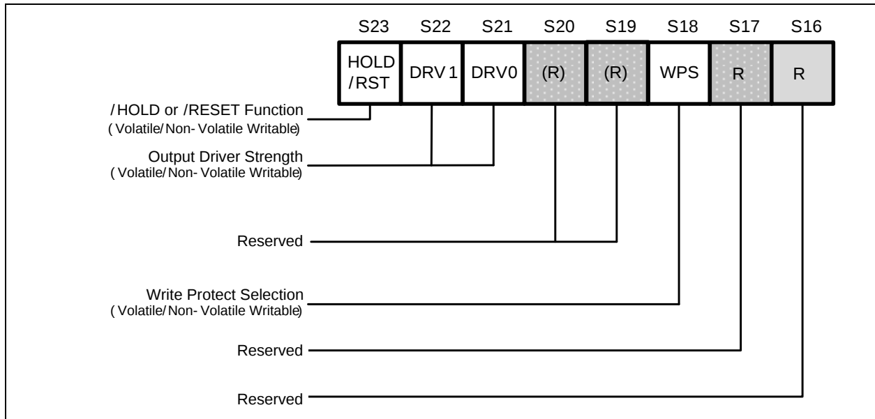
Figure 4c. Status Register-3
