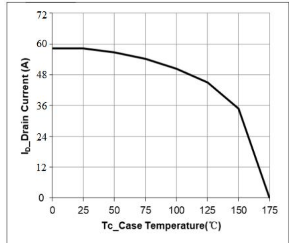
Figure 9 Current De-rating
