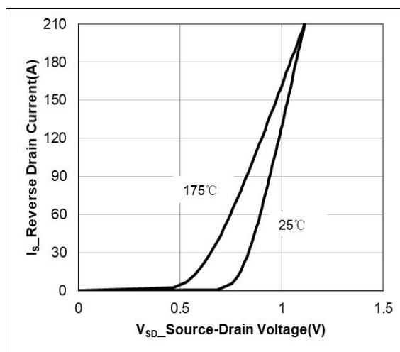
Figure 6 V_{SD\_} Source-Drain Diode forward
