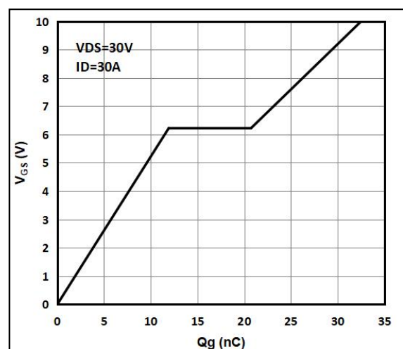
Figure 5 Gate Charge
