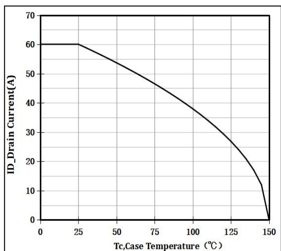
Figure 3 Current De-rating
