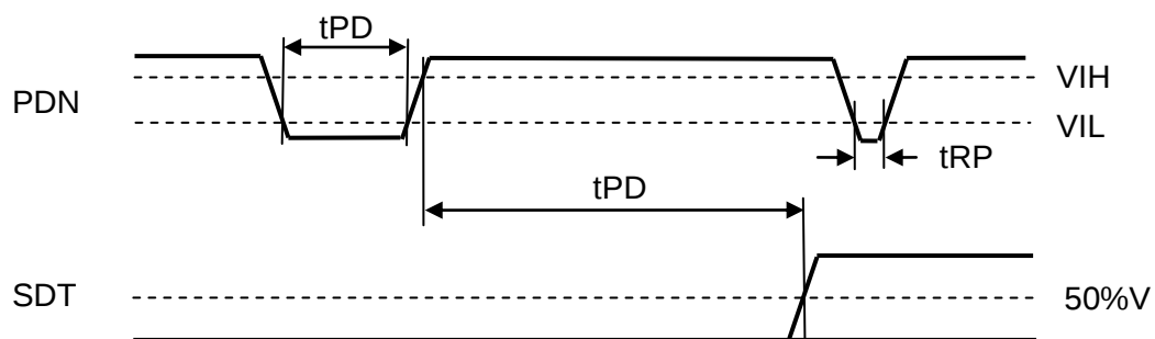
Figure 7. Power-down &amp; Reset Timing
