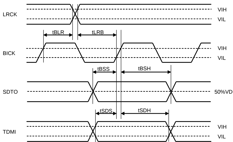
Figure 4. Audio Interface Timing (TDM mode &amp; Slave mode)
