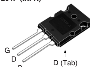
TO-264P (IXFK)
