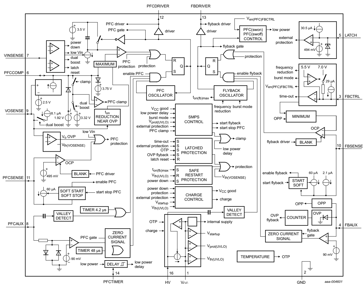
Fig 1. TEA1755LT block diagram
