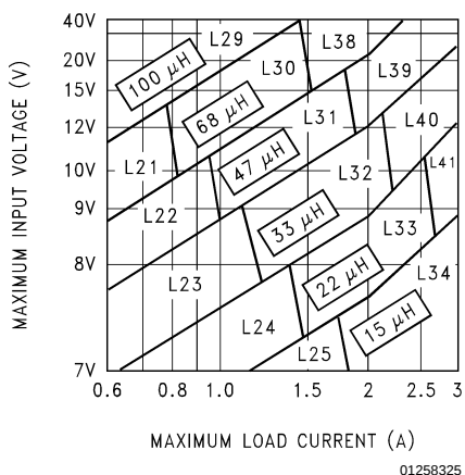
FIGURE 5. LM2596/LM2596HV-5.0
