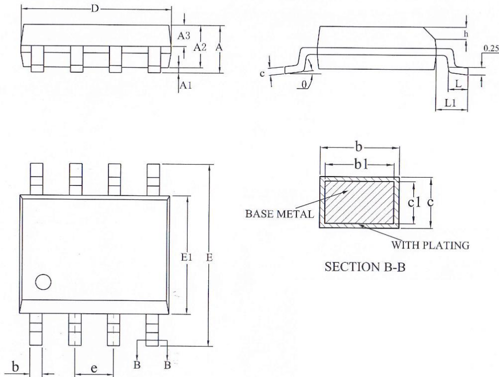
Dimensional In Millimeters
