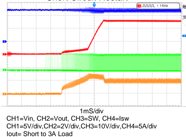
Short Circuit Restart
