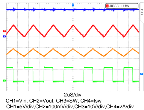
5A Load Test
