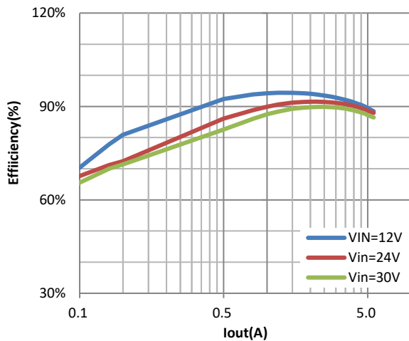
Efficiency &amp; Iout (%)
