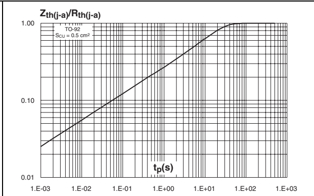
Figure 6. Relative variation of thermal impedance junction to ambient versus pulse duration (PCB FR4, copper thickness = 35 \mu\text{m} , S_{\text{CU}} = 0.5 \text{ cm}^2 ) (TO-92)
