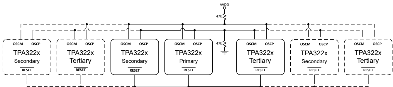
Figure 9-6. Gain and Primary PCB Implementation
