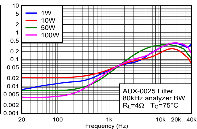
Figure 10-3. Total Harmonic Distortion+Noise vs Frequency
